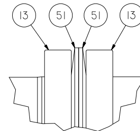
VERY IMPORTANT DRAWING OF ASSEMBLING BELLEVILLE WASHER
